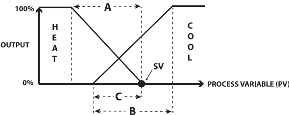
FIGURE 6.5: DEAD BAND (db) SET TO A NEGATIVE NUMBER
