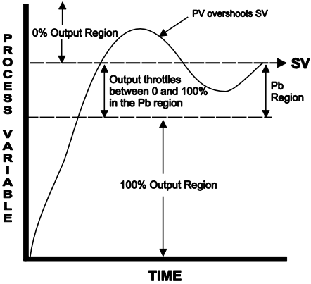
Proportional Band (Pb) set too narrow
