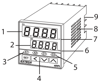
FIGURE 5.2: 48VFL FRONT PANEL
