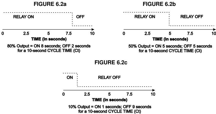
FIGURE 6.2: TIME PROPORTIONING CONTROL EXAMPLES
