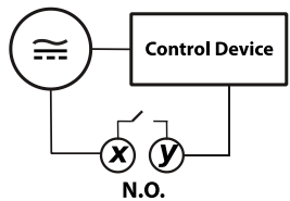
FIGURE 4.2: NORMALLY OPEN (N.O.) CONTROL OUTPUT WIRING
